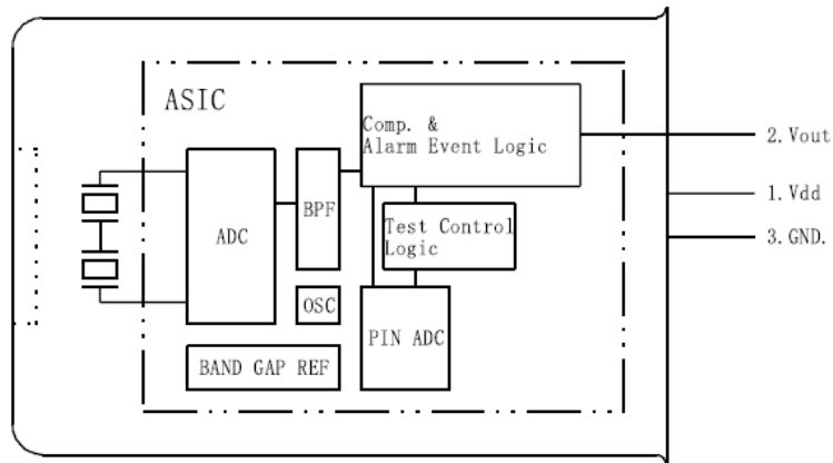
Fig.3:Circuit Configuration
